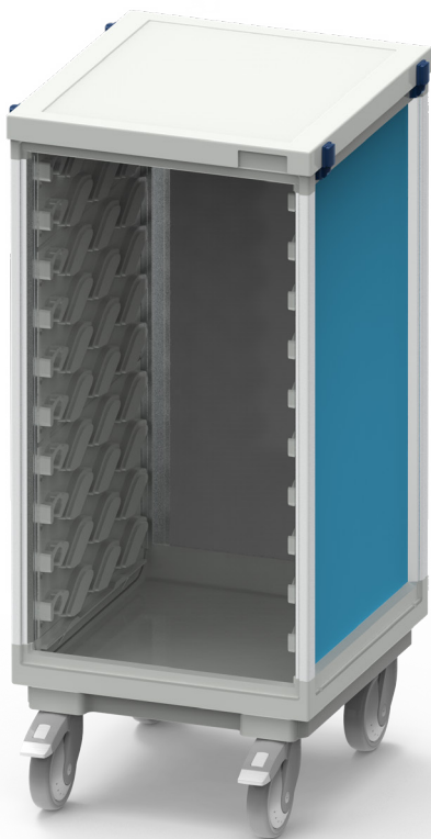
ScanCell® Trolley with Vario liner panels Type D-M075 Item no. 40712000
